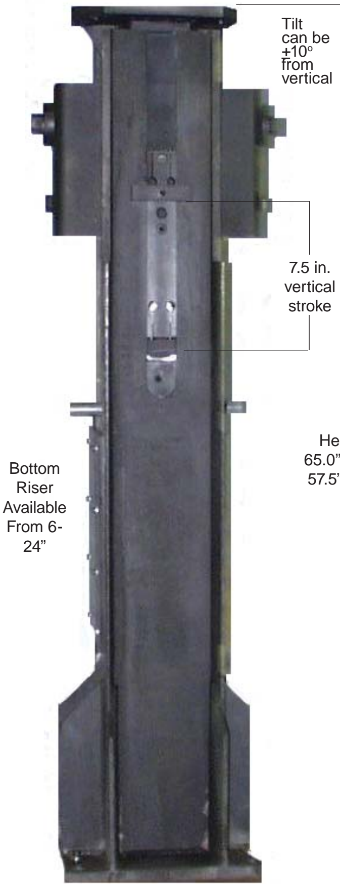
#7770 COMBO TILT PEDESTAL (SL-650, SL-1400, and SL-1500 Only)
